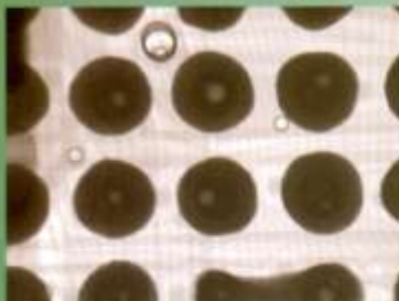
BGA Void X-Ray Image
